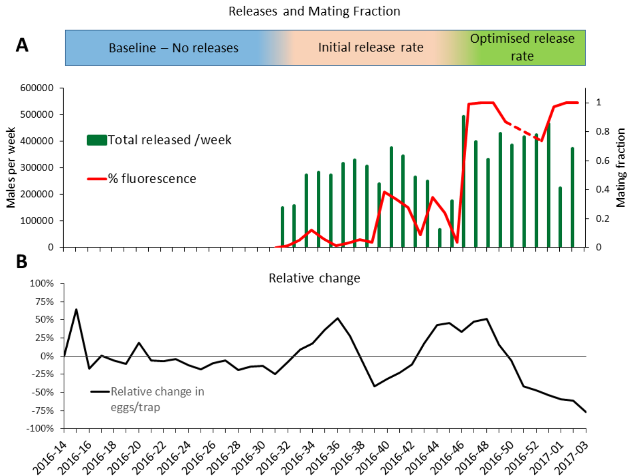
Figure 1: (A) Number OX513A males released per week and Mating Fraction (Percentage of marked fluorescent larvae) observed in the release area of West Bay. The dotted line indicates two missing data points; (B) Relative change in population in the release area relative to the comparator area. A negative value indicates suppression in the release area.
