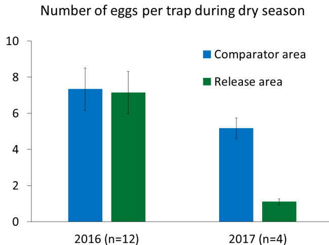
Figure 2: Average number of eggs collected in ovitraps in the release and comparator areas during the dry seasons of 2016 (before OX513A releases) and 2017 (after OX513A releases). A 79% suppression of the Ae. aegypti population was observed between the two periods.
